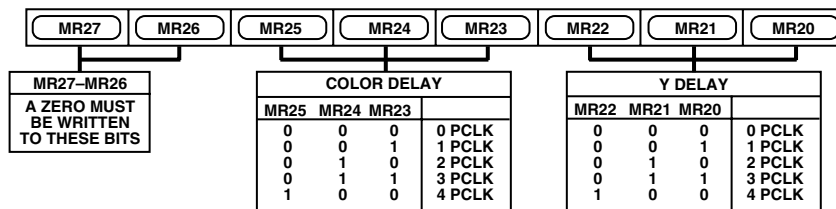
Figure 53. Mode Register 2
